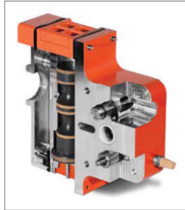
Cutaway of the Wilden® Pro-Flo® SHIFT Air Distribution System (ADS)
